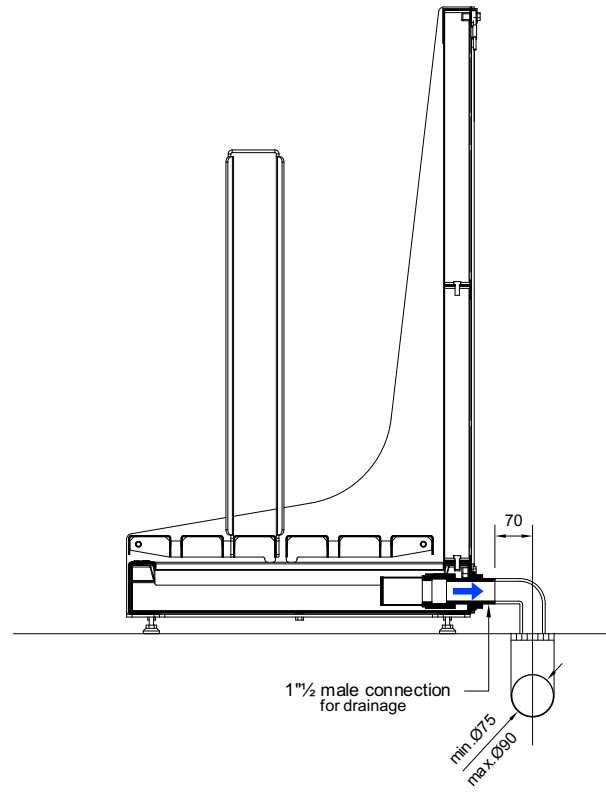
SECTION B-B'
